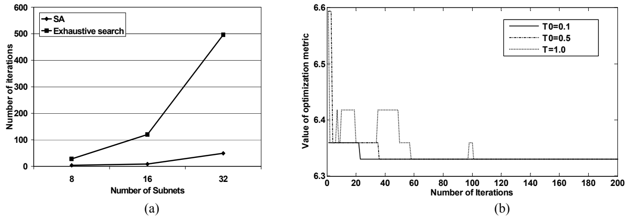
Fig. 5. (a) Number of iterations required to reach optimal solution by the SA and exhaustive search methods (b) Convergence with different temperatures
